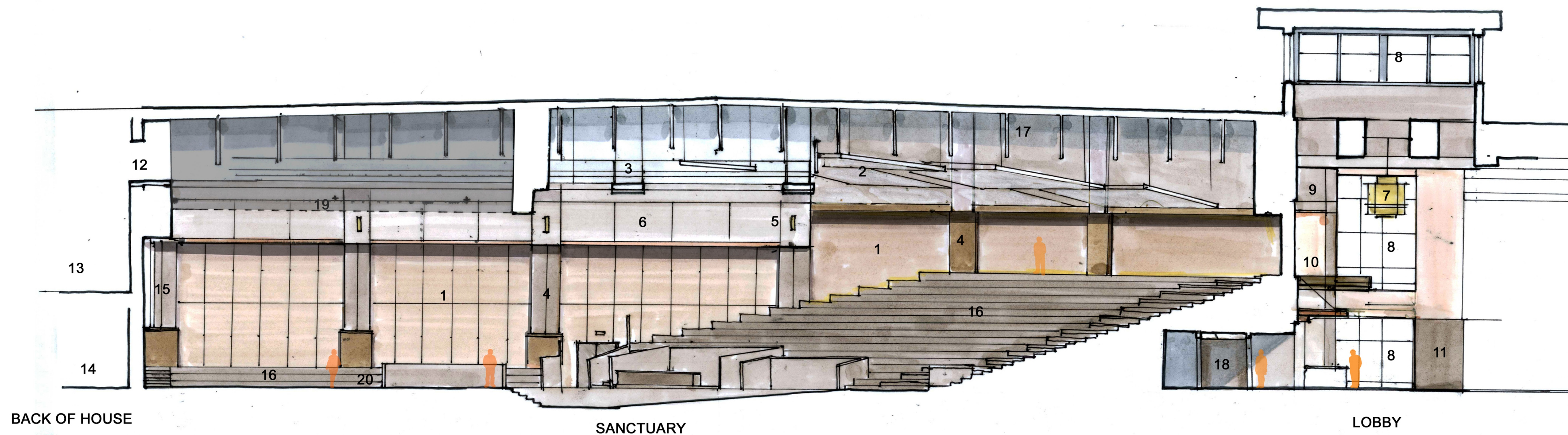
SOUTH WALL INTERIOR ELEVATION
